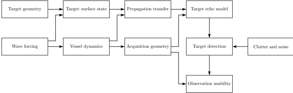
Figure 1: Shared wave forcing drives vessel dynamics and target-surface kinematics. Acquisition geometry and propagation determine the target echo, which is evaluated with clutter and noise by a fixed detector. Observation usability combines detection with corrected position quality, so acquisition geometry also connects directly to the output.
