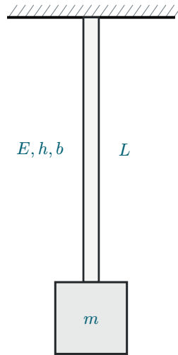
Figure 19: Flex-beam pendulum.
