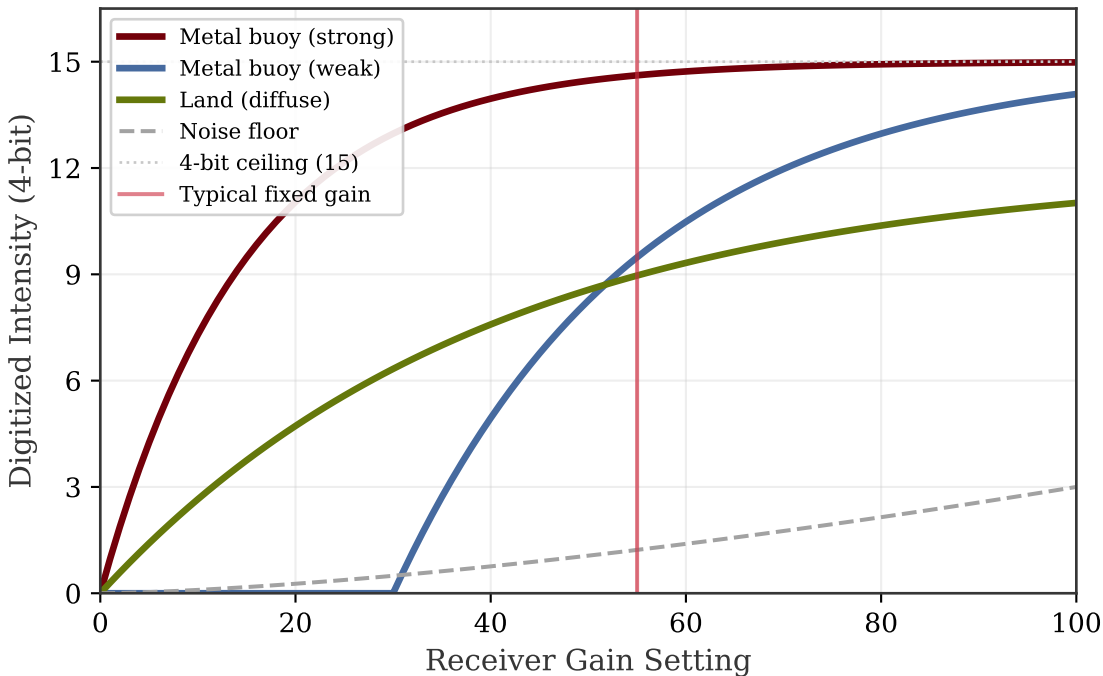
Reflectivity-vs-Gain Response by Target Type
