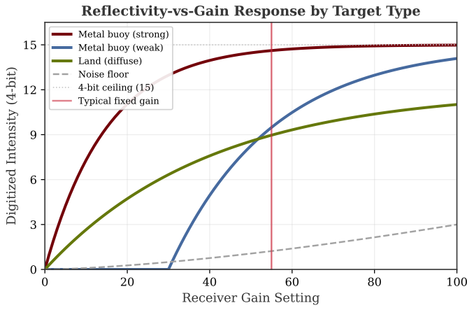
FIGURE 6: Expected reflectivity-versus-gain response curves for three target types. A single fixed gain setting (vertical line) captures only a narrow window of this information. The full gain sweep reconstructs the complete curve, extending effective dynamic range well beyond 4 bits. Placeholder—replace with real measured curves.
