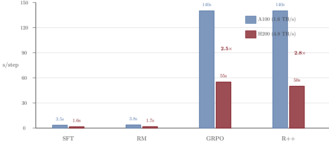
Figure 7: Measured per-step wall time comparison between A100 and H200. SFT and RM are compute-bound with minimal speedup (2.2 \times ). GRPO (2.5 \times ) and R++ (2.8 \times ) are generation-bound, with speedup directly proportional to memory bandwidth ratio. All values measured on Qwen3-8B with identical hyperparameters.
