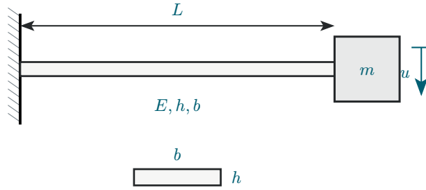
Figure 16: Cantilever beam with tip mass.
