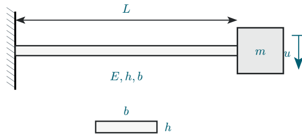
Figure 12: Vertical flex-beam vibrating system.
