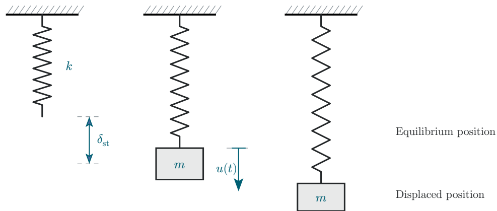
Figure 11: Vertical spring-mass vibration system.
