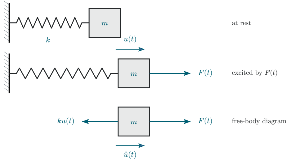
Figure 15: Spring-mass system excited by force F(t) .
