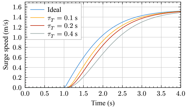
Motor-lag sensitivity
