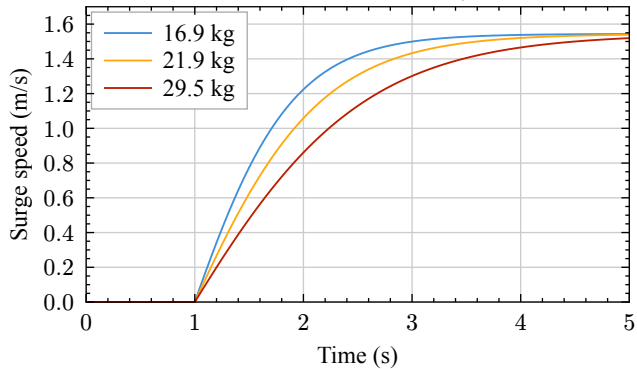
Loaded mass sensitivity
