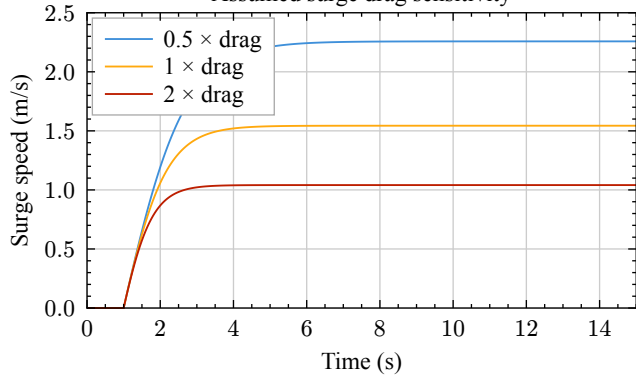
Assumed surge drag sensitivity
