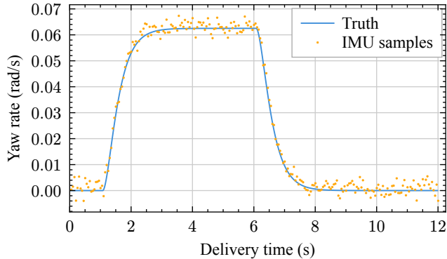
Yaw-rate measurement
