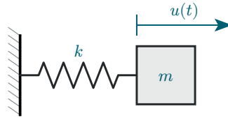
Figure 4: Spring-mass vibrating system.
