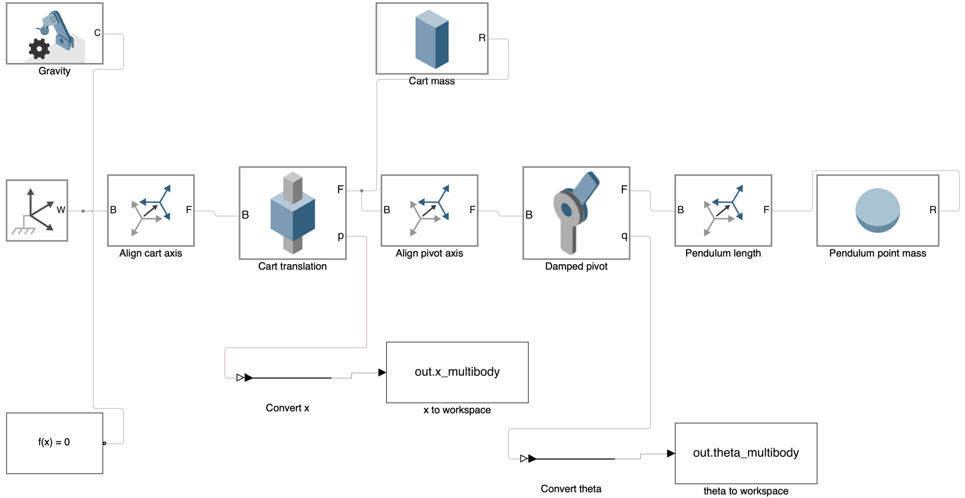
Figure 3: Editable physical-component model with cart translation, gravity, damped pivot, rigid pendulum length, and point mass.
