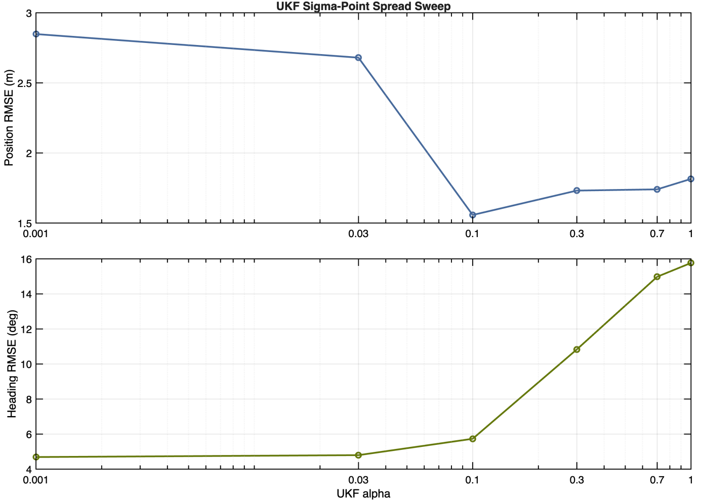
Fig. 9. UKF alpha ablation for the rectangular UKF. The sweep tests whether the reported UKF performance depends on the default narrow sigma-point spread.
