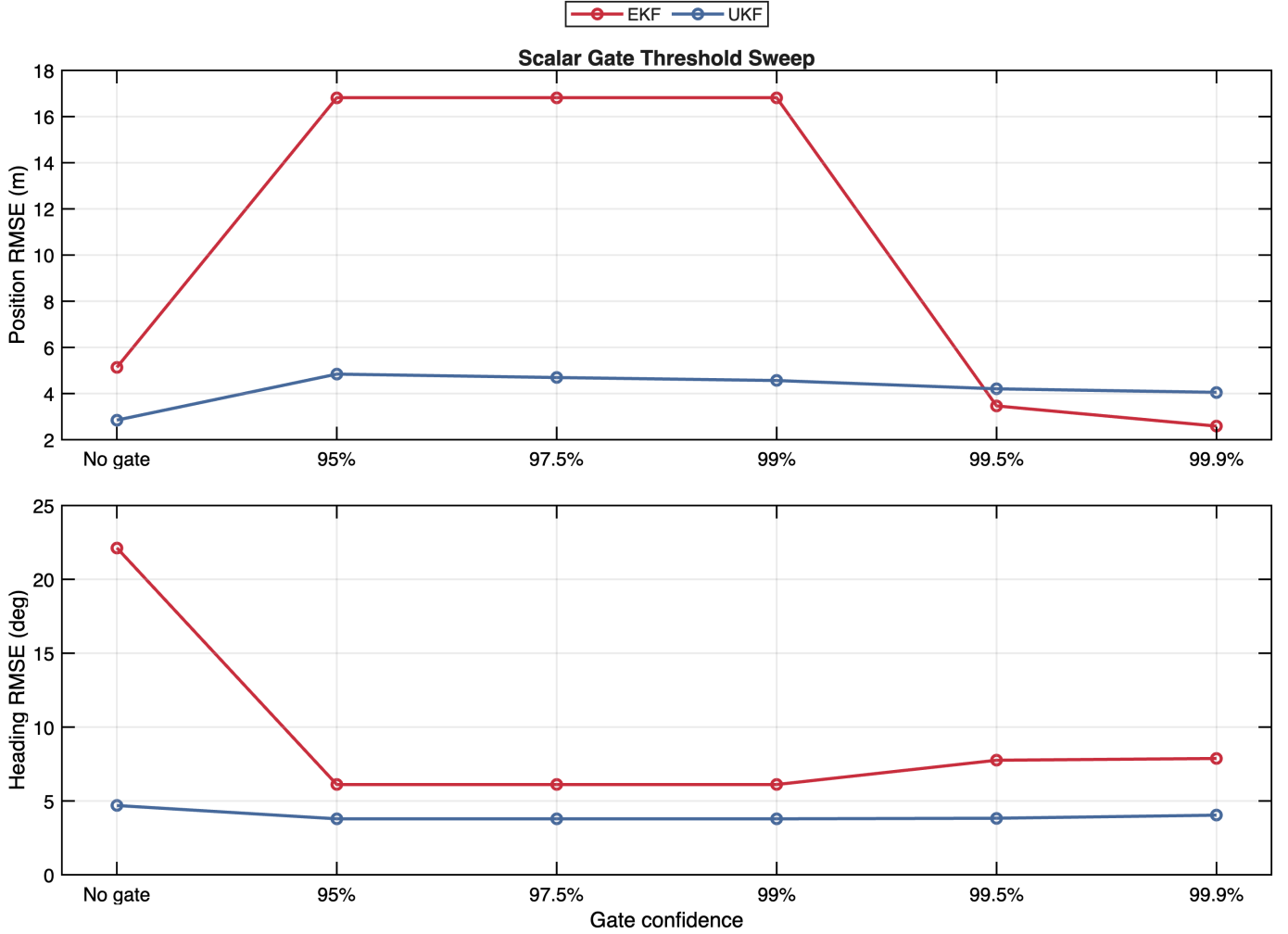
Fig. 6. Gate-threshold ablation for the rectangular EKF and UKF. Position accuracy and heading accuracy respond differently because rejecting late y_1 updates removes radial information, while rejecting isolated y_2 outliers can improve heading.
