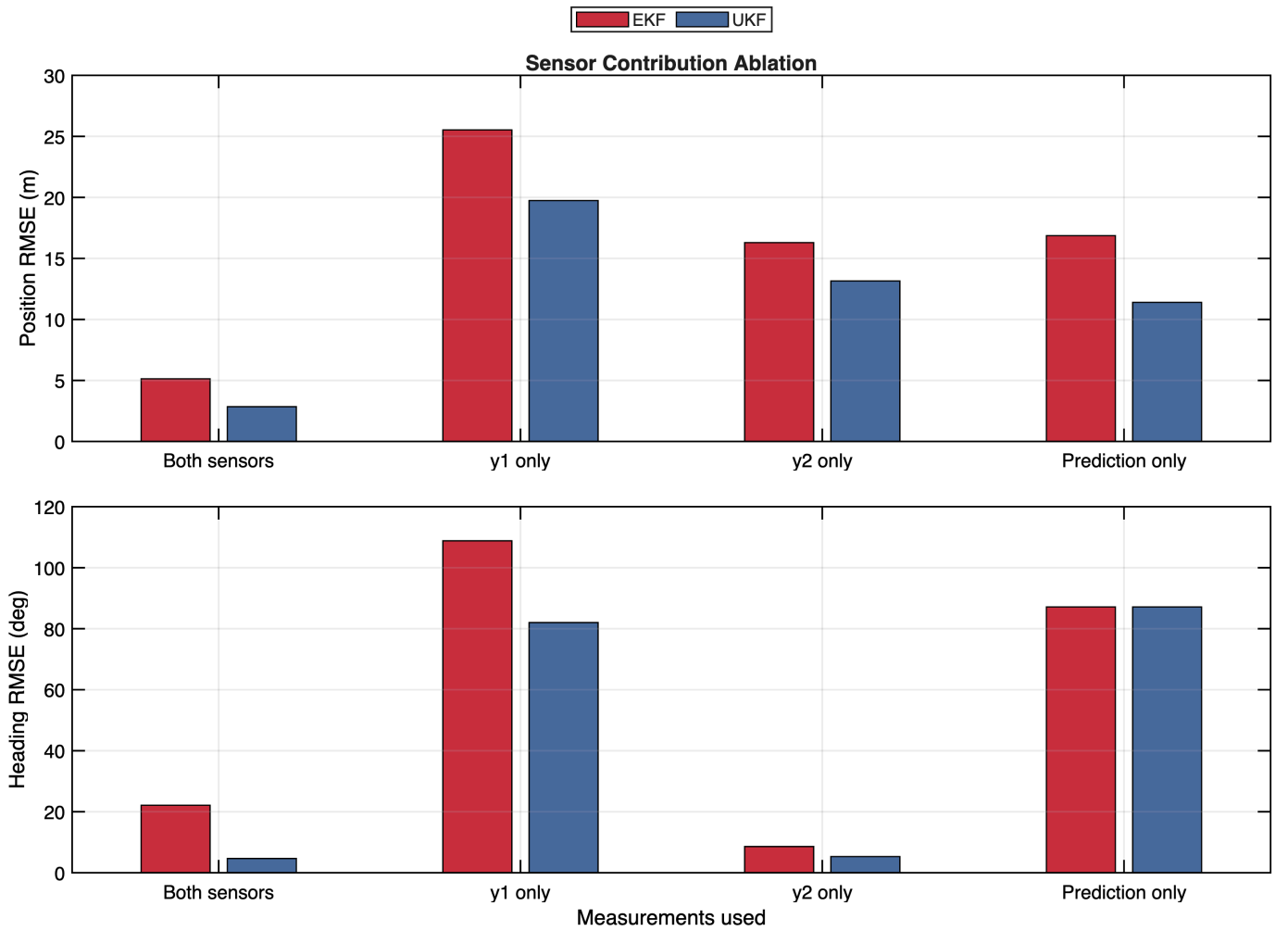
Fig. 7. Measurement-subset ablation for rectangular EKF and UKF runs. The comparison separates radial measurement information from heading measurement information and includes a prediction-only baseline.
