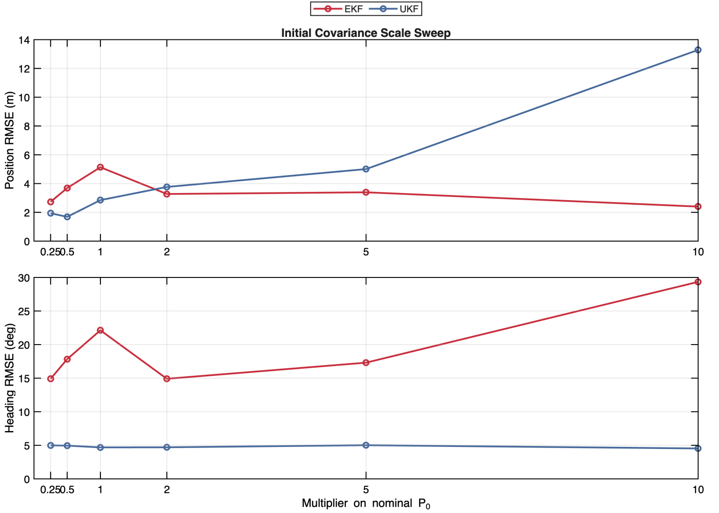
Fig. 8. Initial covariance scale ablation for the rectangular EKF and UKF. The horizontal axis multiplies the nominal P_0 used in the main study.
