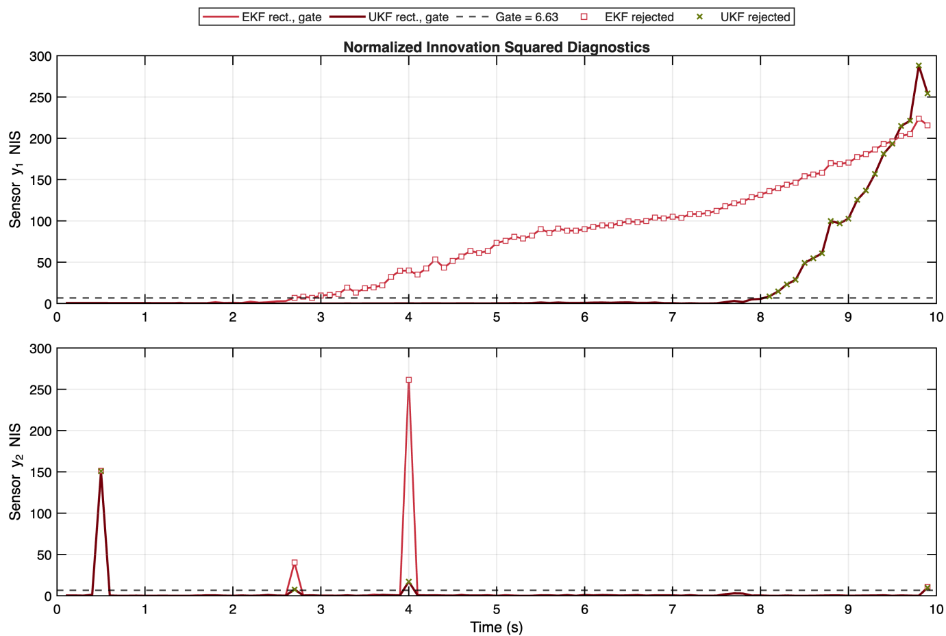
Fig. 4. Normalized innovation squared histories for both scalar sensors. The isolated y_2 spikes are clearly detectable, and the EKF and UKF rejection markers show how the late growth in y_1 residuals drives repeated range-measurement rejection.
