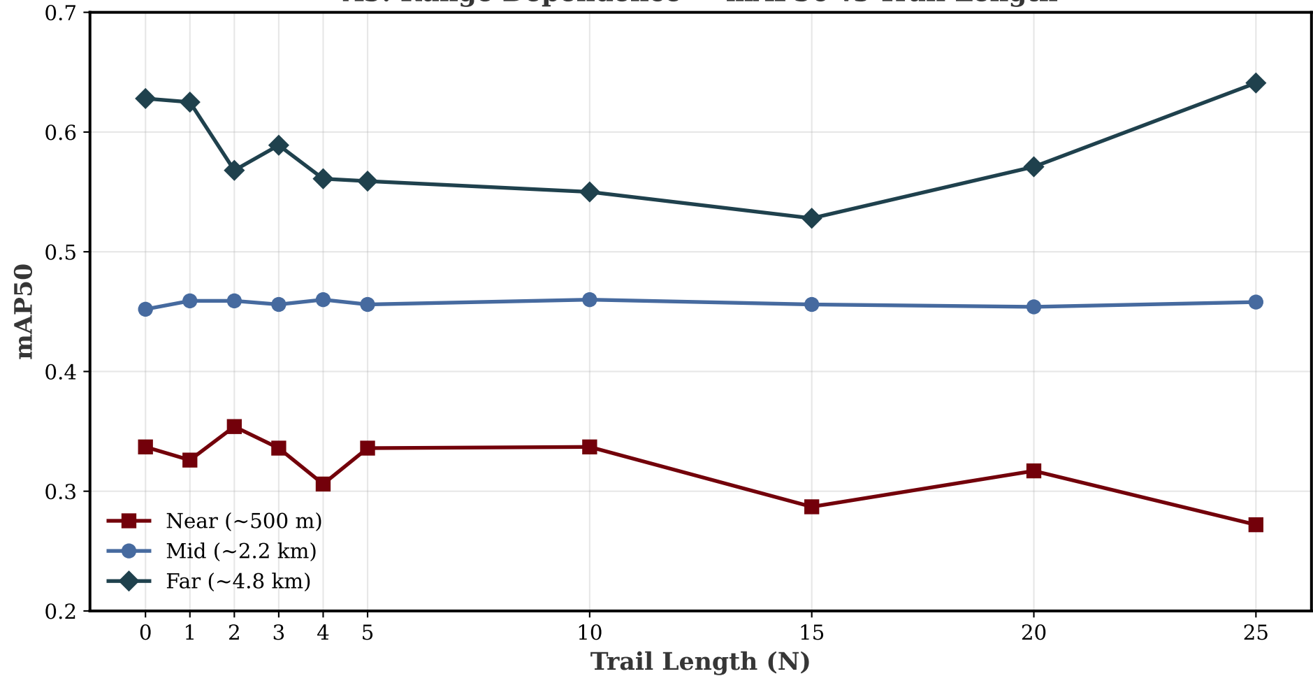
A5: Range Dependence — mAP50 vs Trail Length
