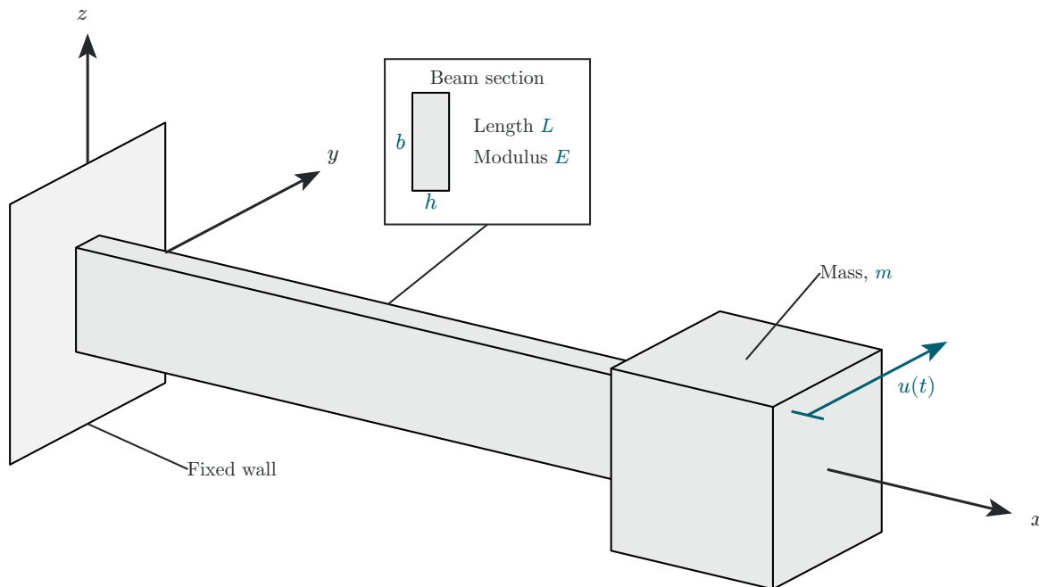
Figure 25: Flex-beam vibrating system.
