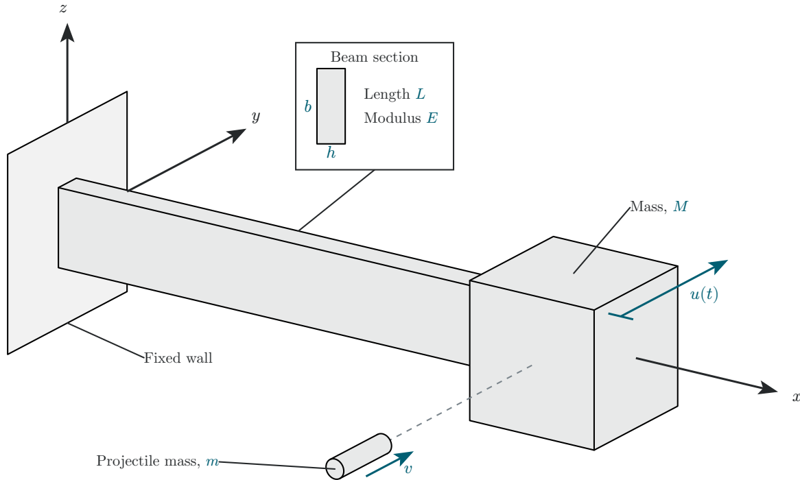
Figure 21: Impact excitation of a horizontal flex-beam vibration system.
