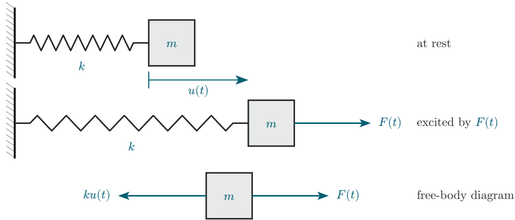
Figure 26: Spring-mass system excited by force F(t) .
