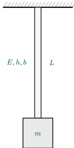
Figure 28: Flex-beam pendulum.
