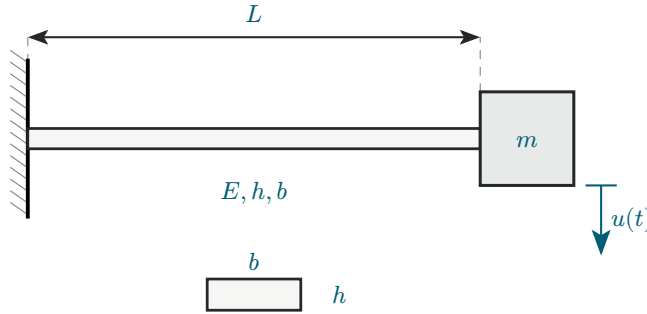
Figure 27: Cantilever beam with tip mass.
