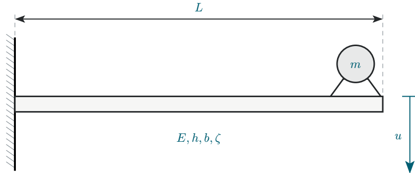
Figure 20: Damped cantilever beam excited by force F(t) from slightly unbalanced electric motor.
