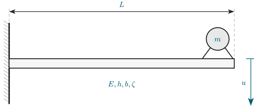
Figure 13: Damped cantilever beam excited by force F(t) from slightly unbalanced electric motor.
