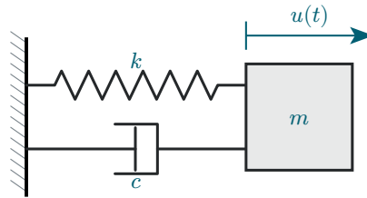
Figure 10: Spring-mass-damper vibrating system.
