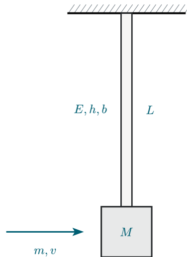
Figure 22: Impact excitation of a vertical flex-beam pendulum.
