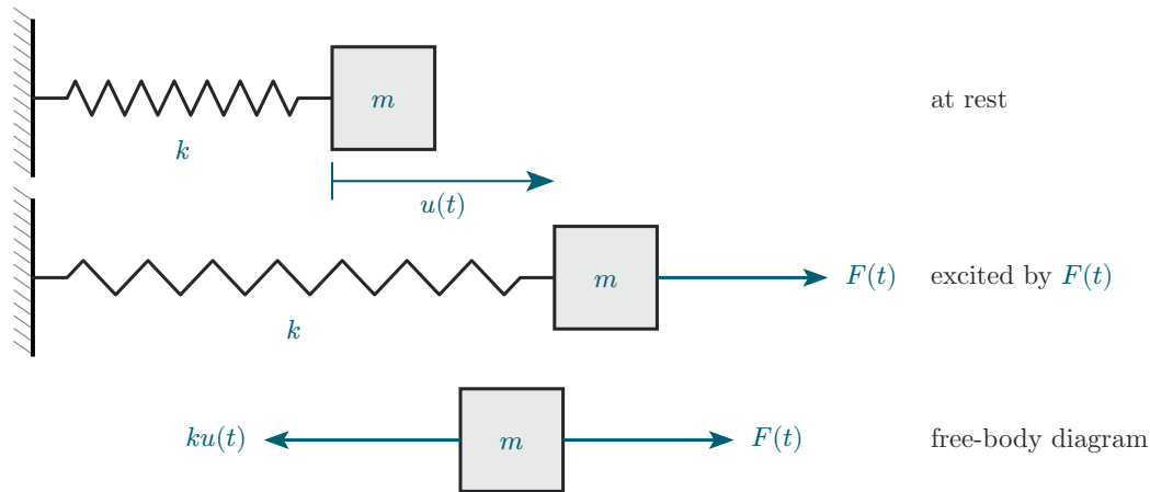
Figure 19: Spring-mass system excited by force F(t) .
