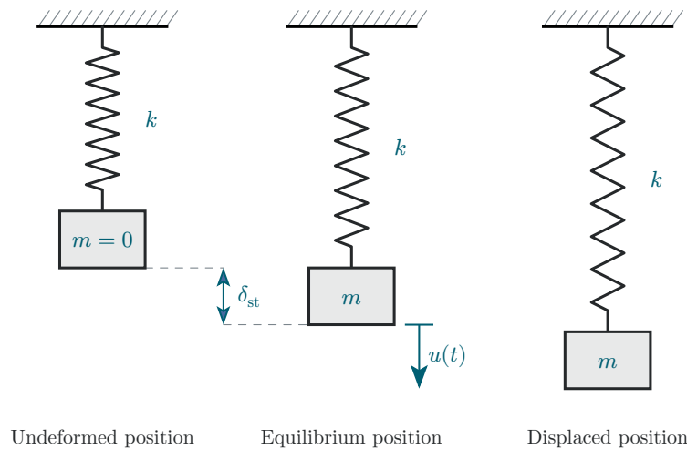
Figure 15: Vertical spring-mass vibration system.
