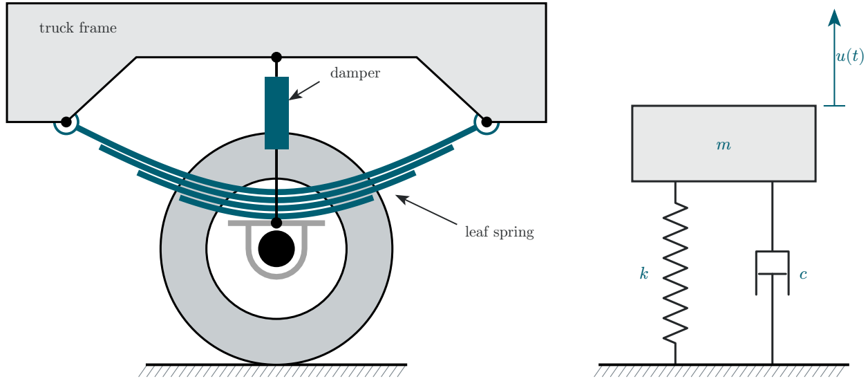
Figure 11: Truck suspension consisting of a leaf spring and an oil damper. The wheel contact is treated as the road datum in the one-degree-of-freedom idealization.
