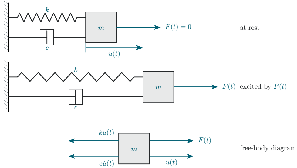
Figure 8: Spring-mass-damper system excited by force F(t) .
