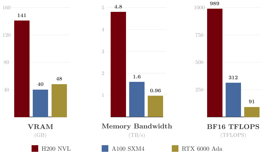
Figure 9: Comparison of available GPU resources. Memory bandwidth, not TFLOPS, is the primary determinant of RL training speed because autoregressive generation requires reading the full model weights for every token produced. The H200’s 4.8 TB/s HBM3 bandwidth makes it 3\times faster than A100 and 5\times faster than RTX 6000 Ada for generation-heavy workloads.
