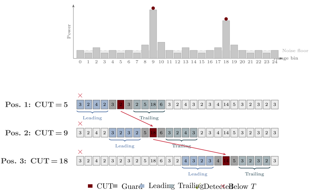
Diagram 1: CFAR Sliding Window
