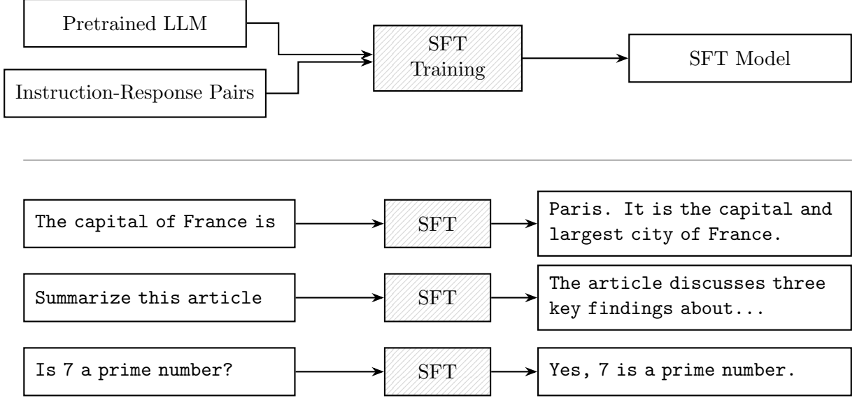
Figure 2: Stage 2: Supervised Fine-Tuning. The pretrained model is fine-tuned on curated instruction-response pairs. The resulting SFT model can follow instructions, summarize text, and answer questions directly.
