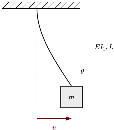
(a) Displaced cantilever
