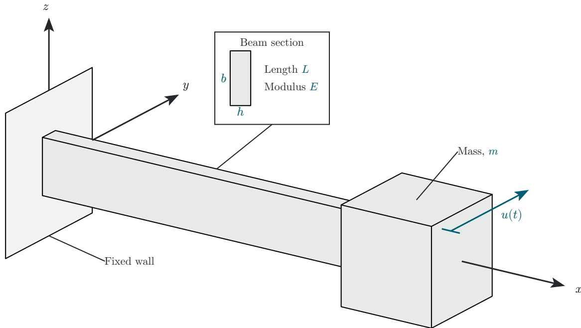
Figure 31: Flex-beam vibrating system.
