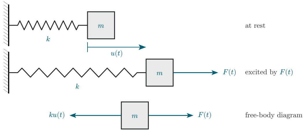
Figure 32: Spring-mass system excited by force F(t) .
