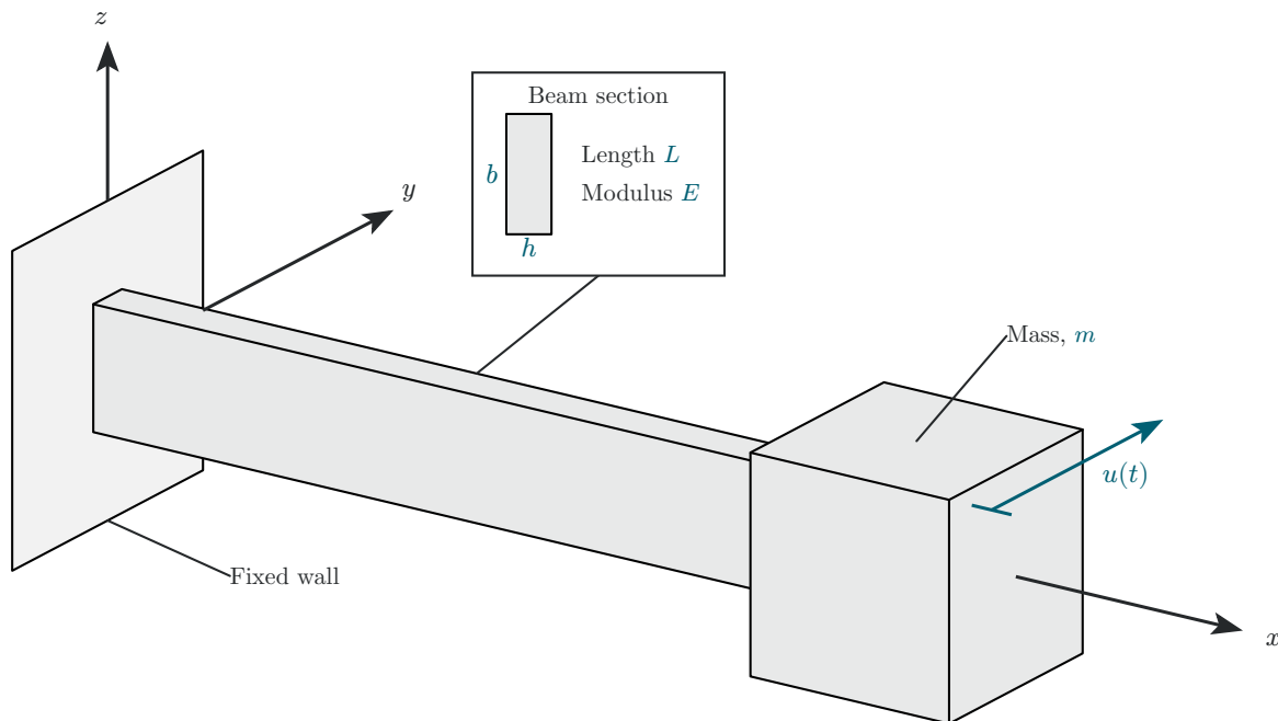
Figure 30: Horizontal flex-beam vibrating system.
