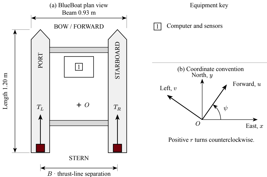
Figure 1: BlueBoat hull plan with the computer and sensors grouped under label 1; O denotes the hull reference origin. B is the surveyed thrust-line separation. The envelope uses published length and beam; the equipment compartment is schematic. The coordinate inset defines \psi and r independently of the bow-up plan.
