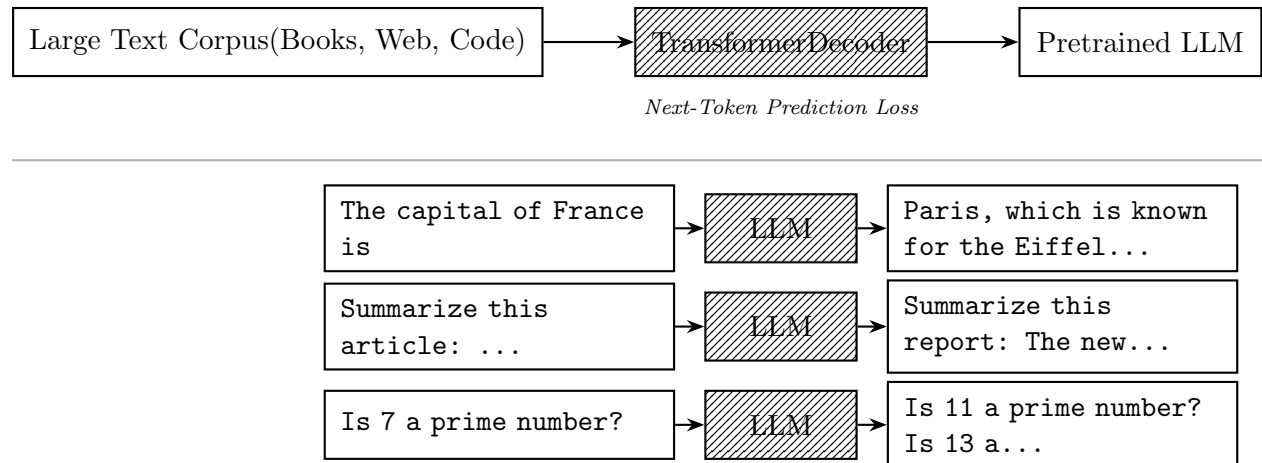
Figure 1: Stage 1: Pretraining. A transformer decoder is trained via next-token prediction on a large text corpus. The resulting model excels at text completion but cannot follow instructions or answer questions, as shown in the example inputs and outputs below the divider.
