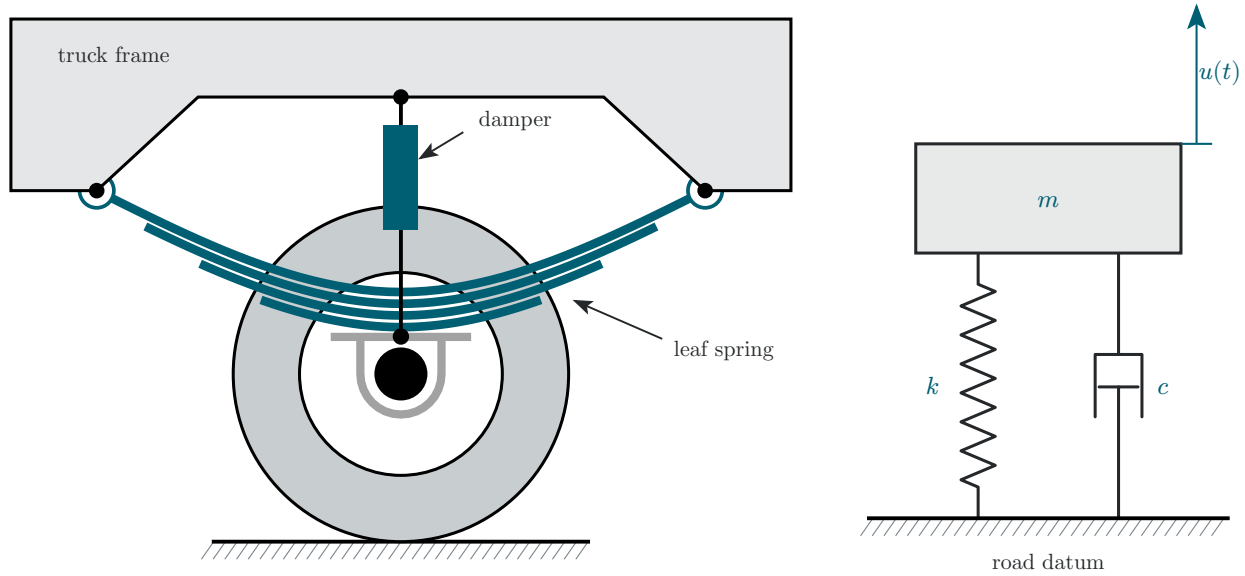
Figure 7: Truck suspension consisting of a leaf spring and an oil damper. The wheel contact is treated as the road datum in the one-degree-of-freedom idealization.
