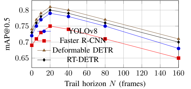
Fig. 3. Accuracy–horizon curves showing an optimal medium trail length and degradation under long trails.
