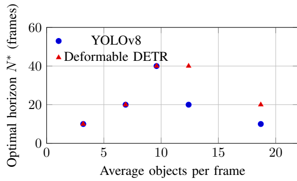
Fig. 5. Cross-location trend: optimal horizon varies with density and occlusion.
