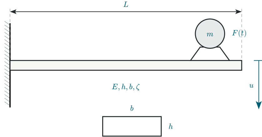
Figure 9: Damped cantilever beam excited by force F(t) from slightly unbalanced electric motor.
