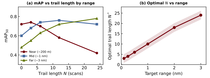
FIGURE 5: mAP_{50} vs. trail length at three target ranges for moving targets at the same physical speed. Near-range targets produce large pixel displacement per scan and prefer short trails; far-range targets produce small displacement and prefer long trails. Placeholder—replace with experimental data.
