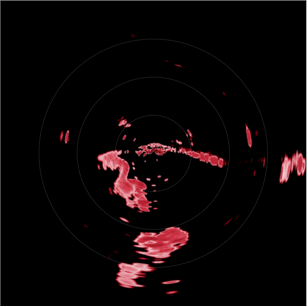
HDR Composite (log)
