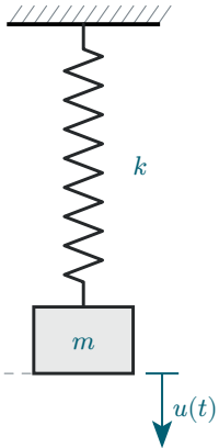
Equilibrium position
