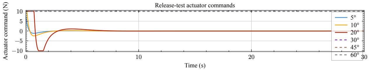
Figure 15: Original initial-angle actuator histories. The failed cases remain at the actuator limit.
