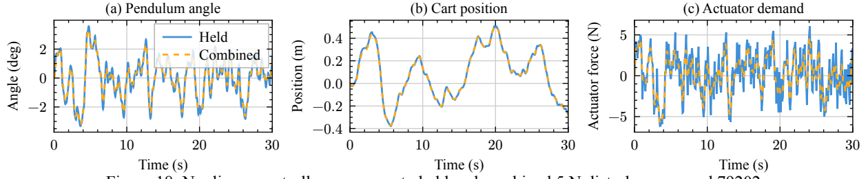
Figure 18: Nonlinear controller responses to held and combined 5 N disturbances, seed 79202.
