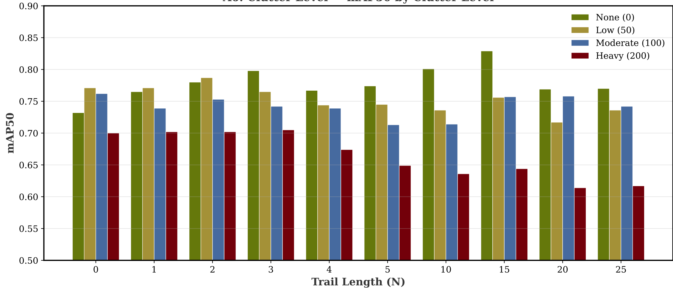
A6: Clutter Level — mAP50 by Clutter Level
