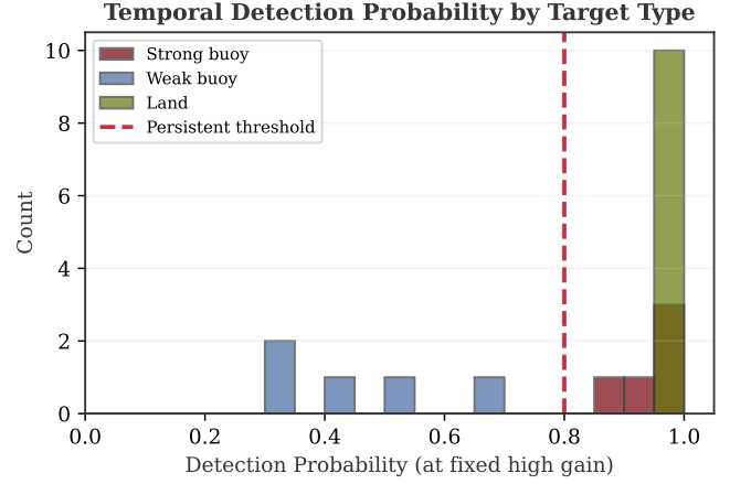
Figure 9: Expected distribution of detection probabilities across target types at fixed high gain over 200 consecutive scans. Weak buoys exhibit lower, more variable detection rates, enabling temporal separation from persistent targets. Placeholder—replace with measured detection probabilities.
