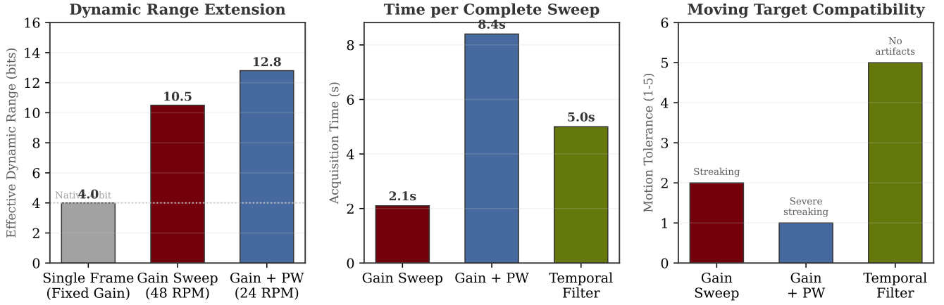
Figure 12: Quantitative comparison of the three gain management strategies. Left: effective dynamic range achieved beyond the native 4-bit resolution. Center: total acquisition time for a complete parameter sweep. Right: tolerance to moving targets on a qualitative scale. Placeholder—replace with measured values.
