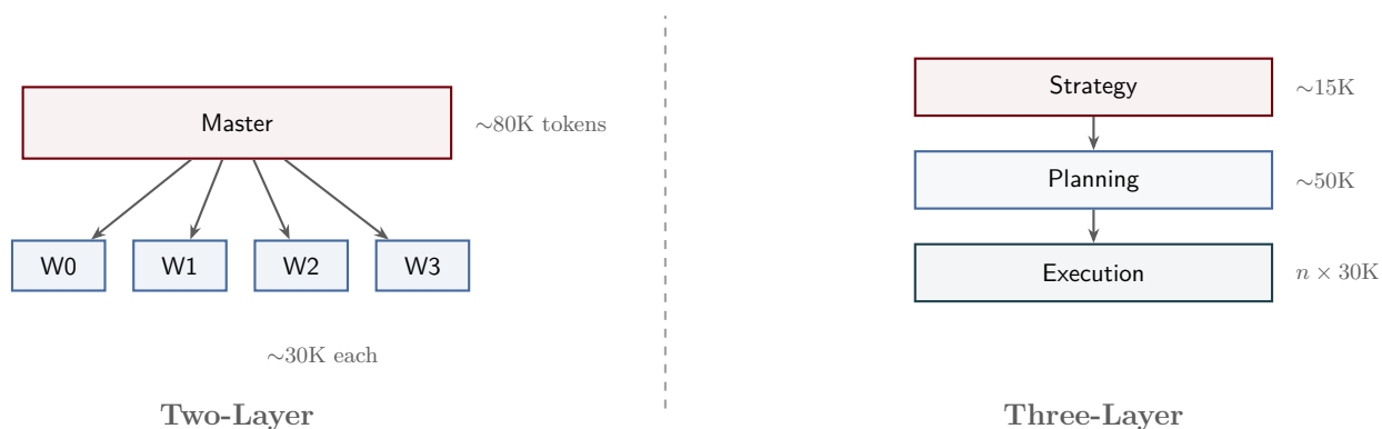
Figure 25: Comparison of two-layer and three-layer agent architectures. The two-layer system places all strategic and tactical reasoning in a single master, consuming a large context budget. The three-layer system separates strategy from planning, allowing each layer to operate within a smaller, more focused context window. The execution layer scales horizontally by adding slaves as needed.
