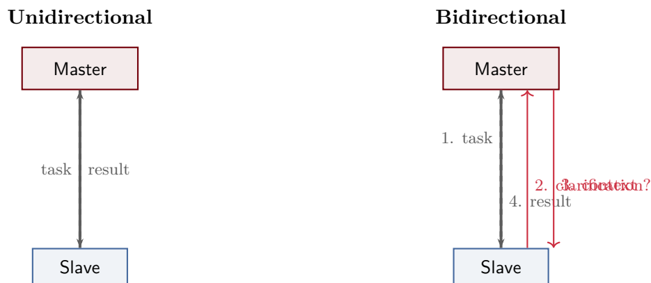
Figure 22: Unidirectional communication (left) vs. bidirectional communication (right). Bidirectional slaves can request clarification mid-task.
