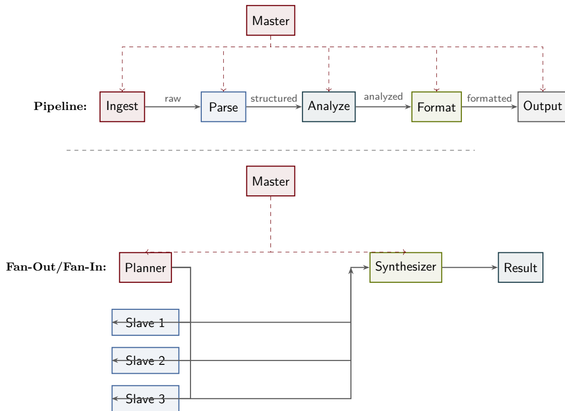
Figure 28: Top: The pipeline pattern processes data through a sequential chain of transformations. Each stage performs a specific operation and forwards the result to the next stage. The master coordinates the chain but does not participate in data transformation. Bottom: The fan-out/fan-in pattern distributes independent subtasks to parallel slaves. The planner decomposes the problem, slaves execute in parallel, and the synthesizer merges results.
