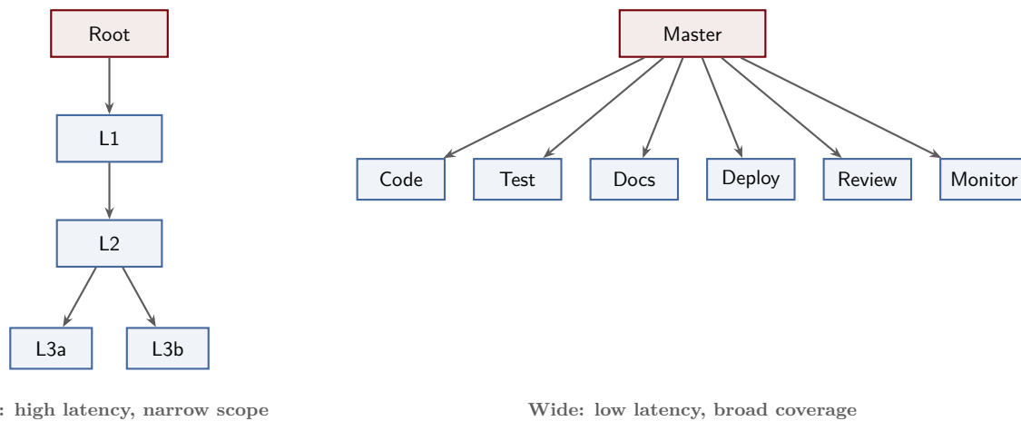
Figure 27: Deep versus wide agent architectures. Deep systems have many layers with narrow branching, resulting in high latency due to sequential handoffs. Wide systems have few layers with broad branching, allowing parallel execution across specialized domains. Each approach has its place: depth for complex decomposition, width for domain coverage.
