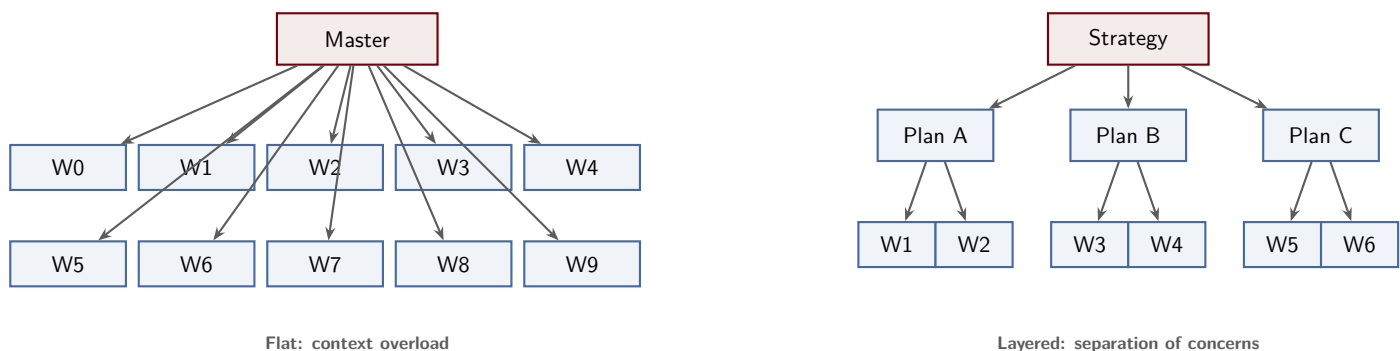
Figure 24: Flat versus layered agent architectures. In flat systems, the master agent must coordinate directly with every worker, leading to cluttered communication and context overload. Layered systems introduce intermediate planning agents that partition the coordination problem into manageable sub-problems.
