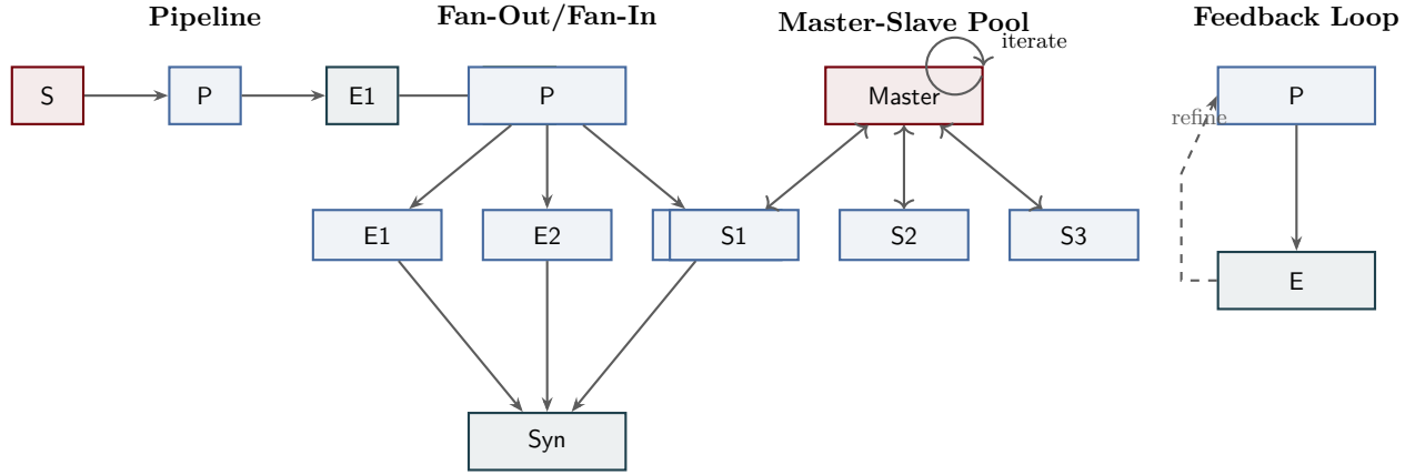
Figure 23: Four canonical orchestration patterns. Each combines topology, orchestration mode, and communication direction in a distinct way.
