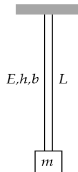
Figure 17: flex-beam pendulum
