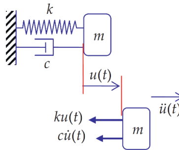
Figure 5 mass-spring-damper vibrating system
