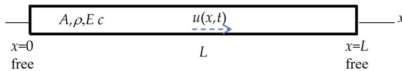
Figure 11 Vibration of a slender bar of finite length L free at both ends
