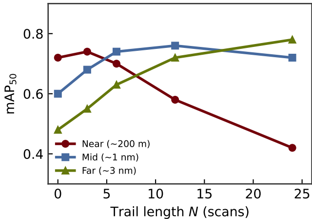
(a) mAP vs trail length by range
