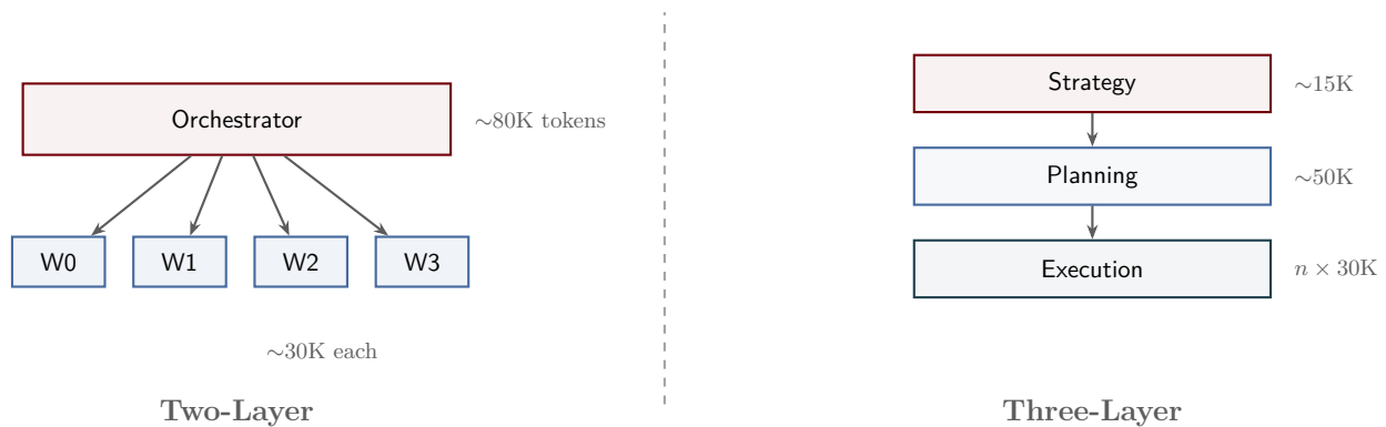
Figure 25: Comparison of two-layer and three-layer agent architectures. The two-layer system places all strategic and tactical reasoning in a single orchestrator, consuming a large context budget. The three-layer system separates strategy from planning, allowing each layer to operate within a smaller, more focused context window. The execution layer scales horizontally by adding workers as needed.
