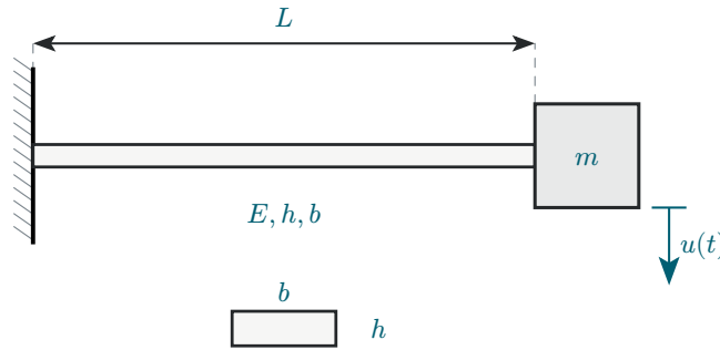
Figure 24: Cantilever beam with tip mass.
