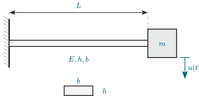
Figure 20: Vertical flex-beam vibrating system.
