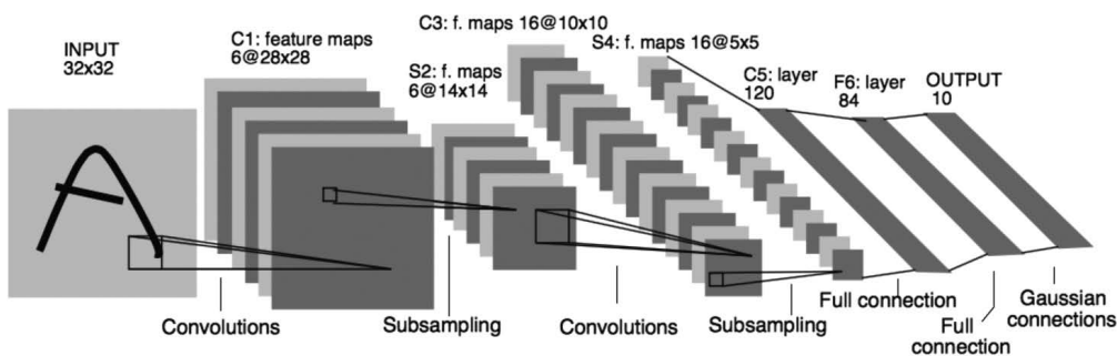
Figure 9.15: Deep Convolutional Network. Republished with permission of Proceedings of the IEEE, from Gradient-based learning applied to document recognition , LeCun, Bottou, Bengio, and Haffner, volume 86, 1998; permission conveyed through Copyright Clearance Center, Inc.
