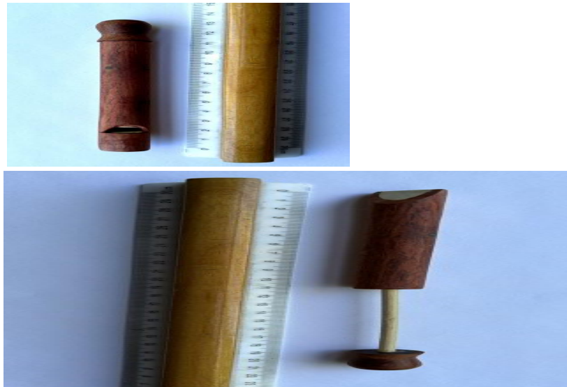
Figure 4: Slide whistle. (a) Fully retracted, showing the piston end. (b) Fully extended. The ruler's major markings are in centimeters.
