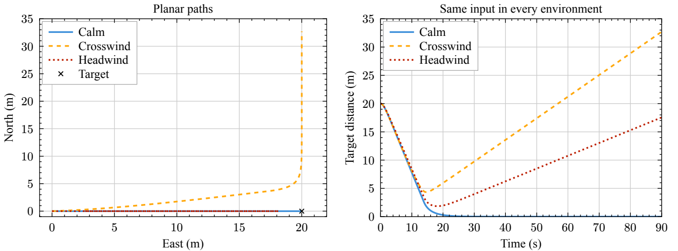
Figure 9: Open-loop target approach in calm water, crosswind, and headwind. Path axes use different scales.
