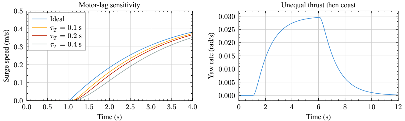
Figure 15: Motor-lag sensitivity and turning response on the slide benchmark plant.
