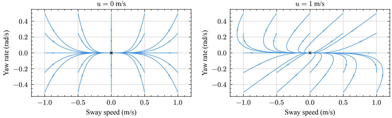
Figure 6: Sway–yaw phase portraits at frozen surge speeds of 0 and 1 m/s.
