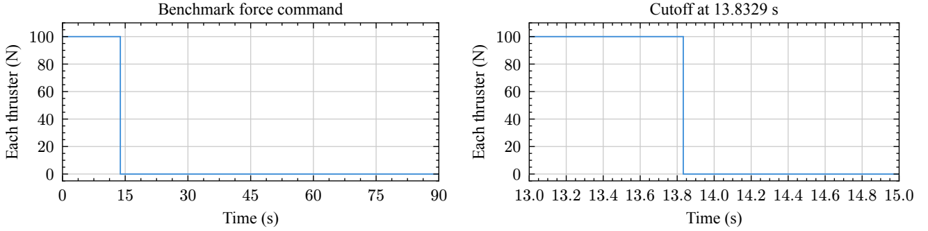
Figure 8: Reconstructed equal-thrust schedule and cutoff detail.
