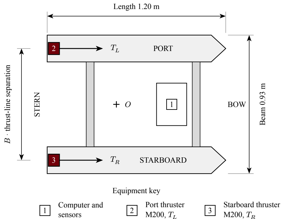
Figure 1: Proposed BlueBoat layout with hull origin O and thrust-line separation B .
