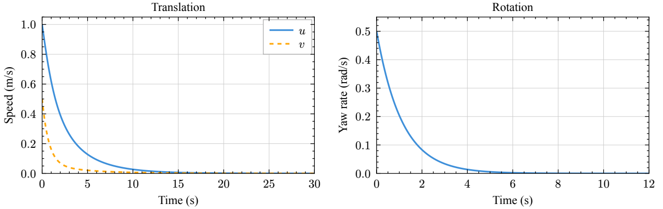
Figure 5: Unforced translation and yaw decay.
