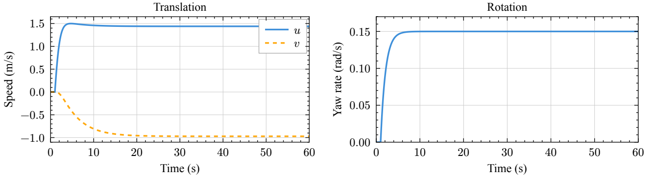
Figure 3: Differential-thrust translation and yaw response.
