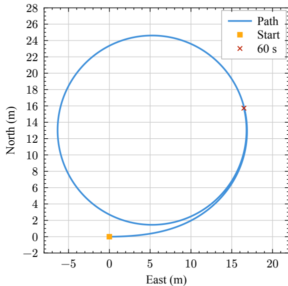
Figure 3: Differential-thrust translation and yaw response.
