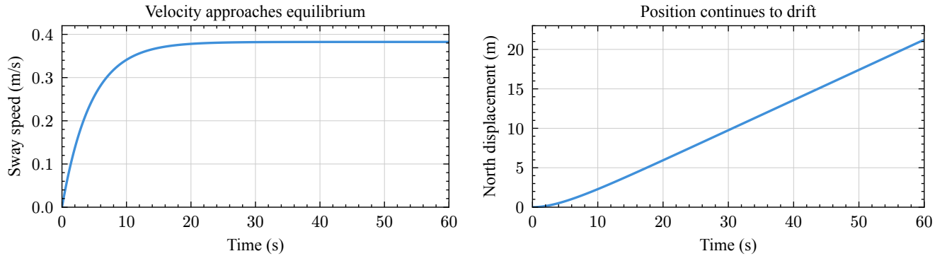
Figure 7: Unpowered crosswind response. Velocity settles while position continues to drift.
