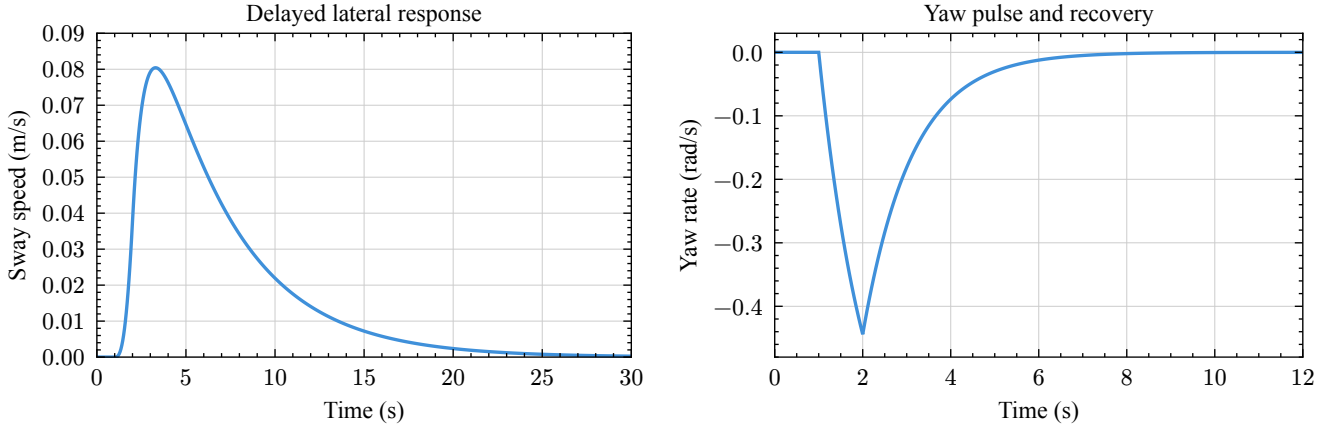
Figure 4: Sway and yaw responses to a one-second thrust pulse.
