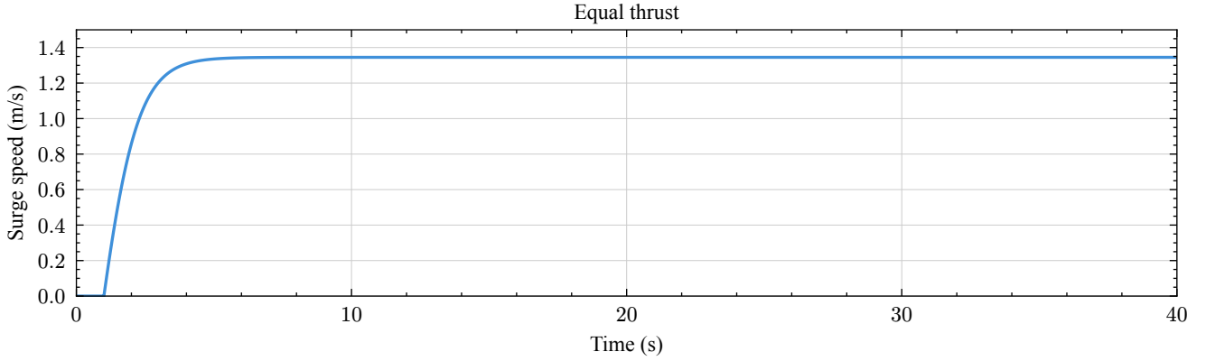
Figure 2: Equal-thrust surge response.
