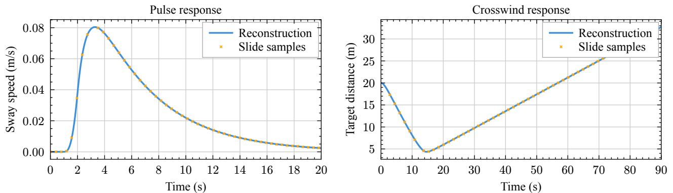
Figure 10: Reconstructed curves against digitized slide samples; every tenth marker is shown.
