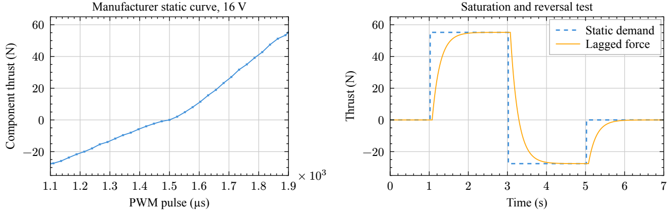
Figure 14: Manufacturer M200 static thrust at 16 V and simulated delayed reversal.
