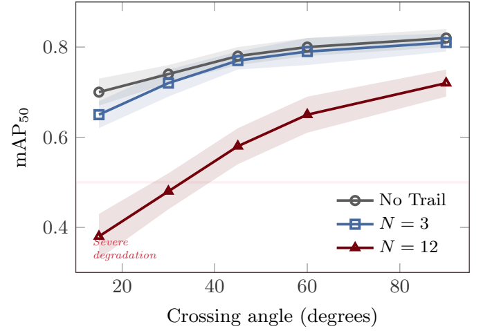
FIGURE 6: mAP_{50} as a function of crossing angle for two moving targets with no trails, short trails ( N = 3 ), and long trails ( N = 12 ). Shallow crossing angles produce extended trail overlap and significant detection degradation. Placeholder—replace with experimental data.
