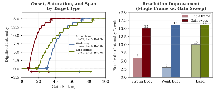
FIGURE 7: Expected onset and saturation points for targets of different reflectivity. The onset-to-saturation span S and the resolution improvement factor R = L/16 quantify the gain sweep's benefit without assuming a dB calibration. Placeholder—replace with measured values.
