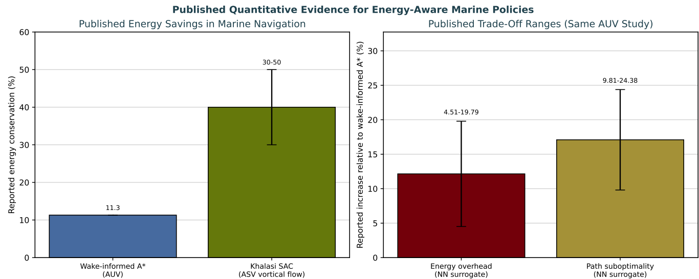
Fig. 3. Published quantitative evidence motivating Proposal 3. Left: reported marine energy-conservation gains from wake-aware and flow-aware planning methods. Right: reported trade-off ranges when replacing wake-aware optimization with learned surrogates.
