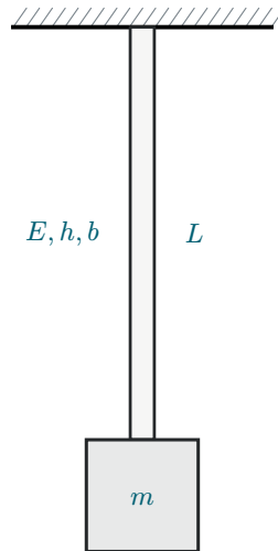
Figure 39: Flex-beam pendulum.
