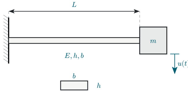
Figure 38: Cantilever beam with tip mass.
