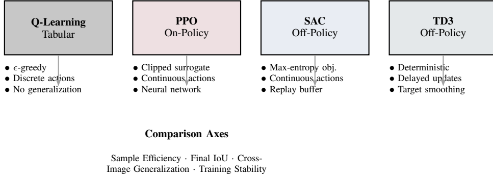
Fig. 4: Comparison of four RL approaches for prompt optimization. The original tabular Q-learning [2] uses discrete graph operations without cross-image generalization. Our proposed deep RL alternatives (PPO, SAC, TD3) use neural network policies with continuous action spaces for direct coordinate prediction.
