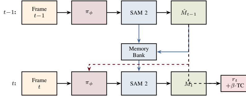
Fig. 3: Temporal prompt optimization with SAM 2. The RL policy receives temporal context from previous frames via the memory bank and prior mask history. The reward includes a temporal consistency (TC) bonus to encourage smooth mask predictions across frames.
