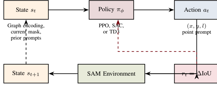
Fig. 2: MDP formulation for RL-based prompt optimization. The state encodes the dual-space graph, current mask, and prior prompts. The policy selects point coordinates and labels. SAM produces a new mask, and the IoU improvement serves as the reward.
