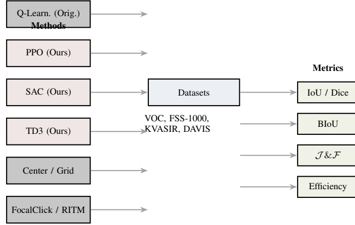
Fig. 5: Evaluation pipeline. RL-based methods (PPO, SAC, TD3) and non-RL baselines are evaluated across four datasets using segmentation quality, boundary accuracy, video tracking, and prompt efficiency metrics.
