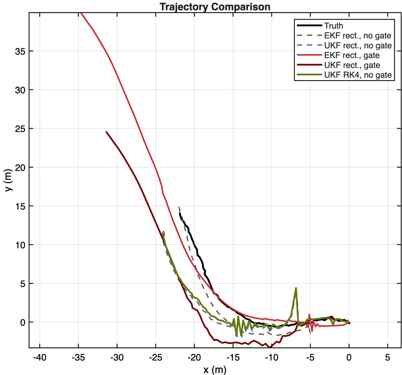
Figure 2: Trajectory comparison for the rectangular EKF and UKF baselines, the gated rectangular filters, and the ungated RK4 UKF. The ungated rectangular EKF gives the lowest position RMSE, while the gated runs drift late in the record after repeated measurement rejection.
