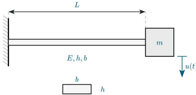
Figure 35: Cantilever beam with tip mass.
