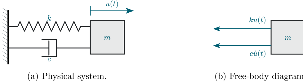
Figure 6: Mass-spring-damper vibrating system.
