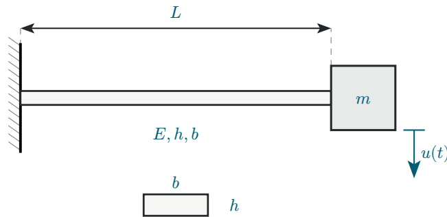
Figure 13: Vertical flex-beam vibrating system.
