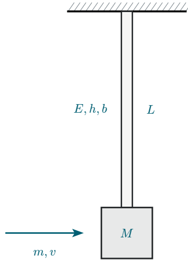
Figure 19: Impact excitation of a vertical flex-beam pendulum.
