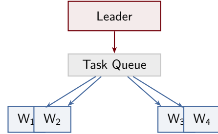
Figure 7: Leader-worker pool with a shared task queue. The leader enqueues tasks; workers dequeue and execute.
