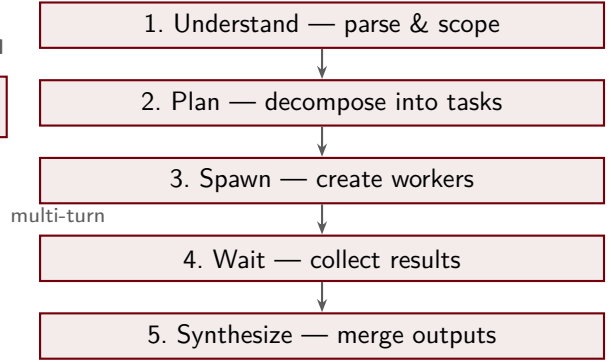
Figure 2: The five-phase orchestrator cycle.
