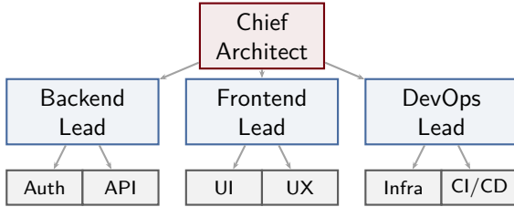
Figure 6: Hierarchical multi-agent system. Domain leads coordinate specialists; the root agent coordinates leads.
