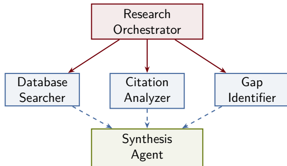
Figure 10: Literature review with three parallel agents feeding a synthesis agent.
