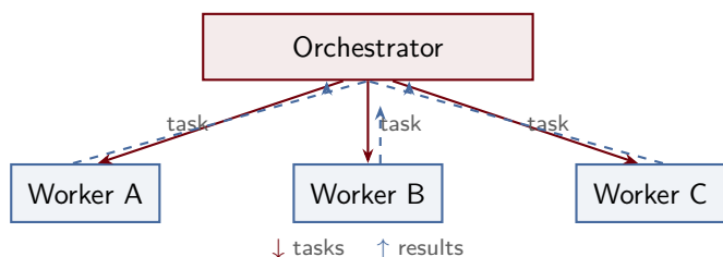
Figure 3: Two-layer communication: the orchestrator delegates tasks downward (solid) and receives results upward (dashed).
