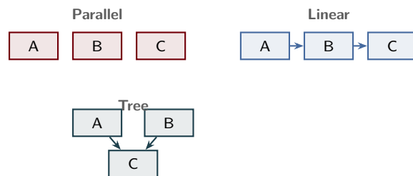
Figure 4: Three canonical dependency patterns for task scheduling.
