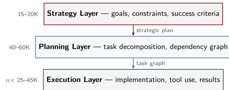
Figure 5: Three-tier architecture with typical token budgets per layer. The execution layer runs multiple agents in parallel.
