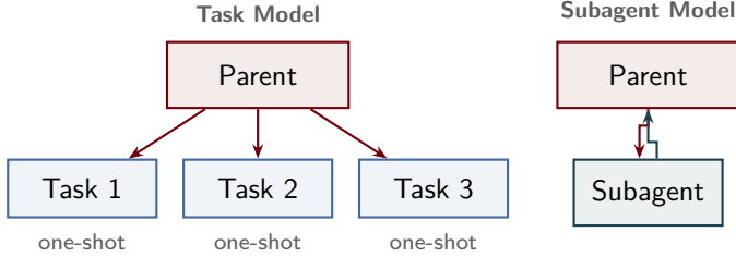
Figure 1: Task (left) vs. subagent (right) delegation. Tasks are one-shot and parallelizable; subagents support iterative dialogue.
